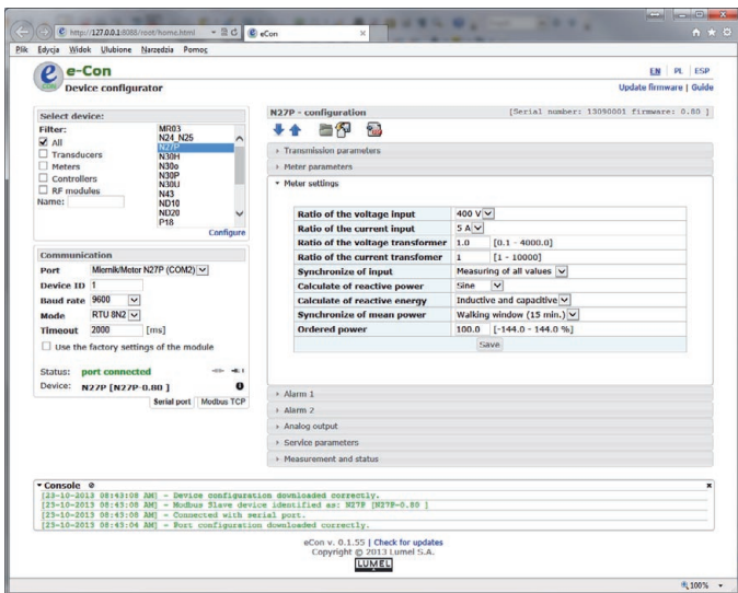
Figure 11. eCon main window
