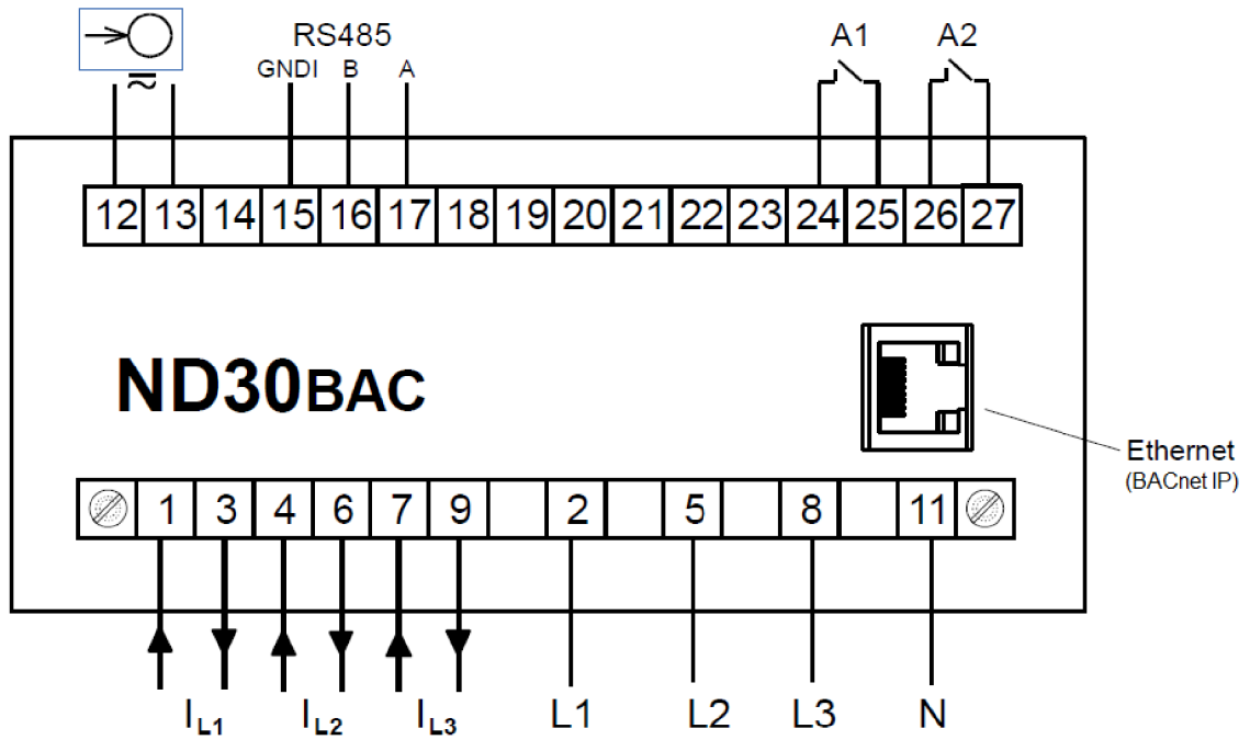
Fig. 4. Meter connections
