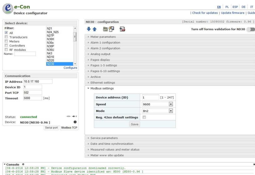
Fig. 25. Program window view: a) eCon, b) software upgrade
