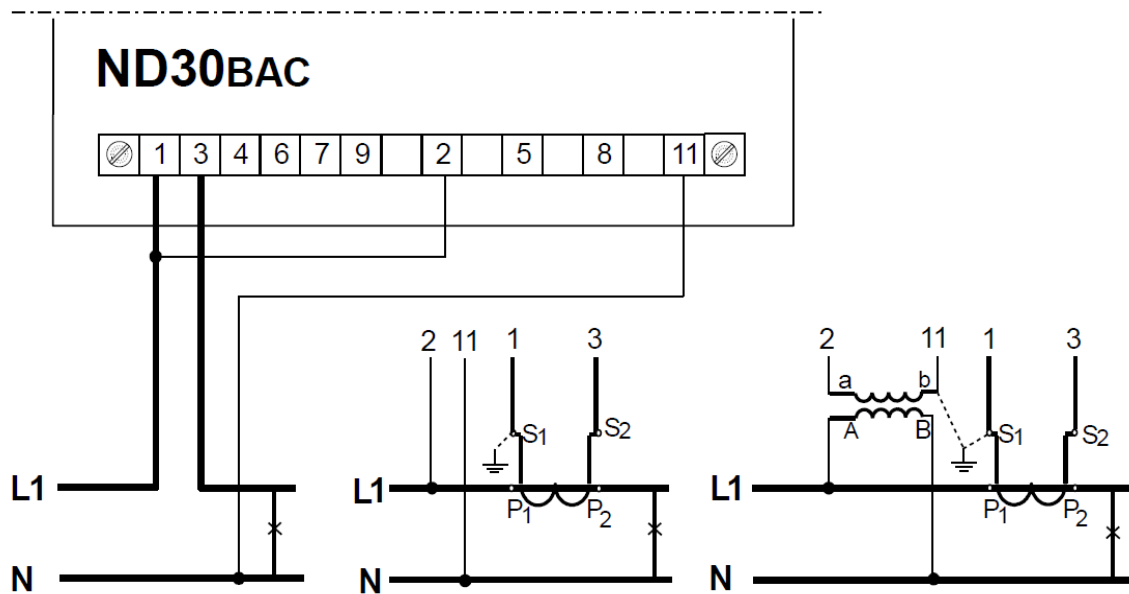
Fig. 4. Meter connections
