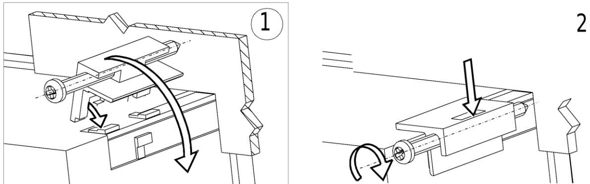
Fig.2. Meter fixing
