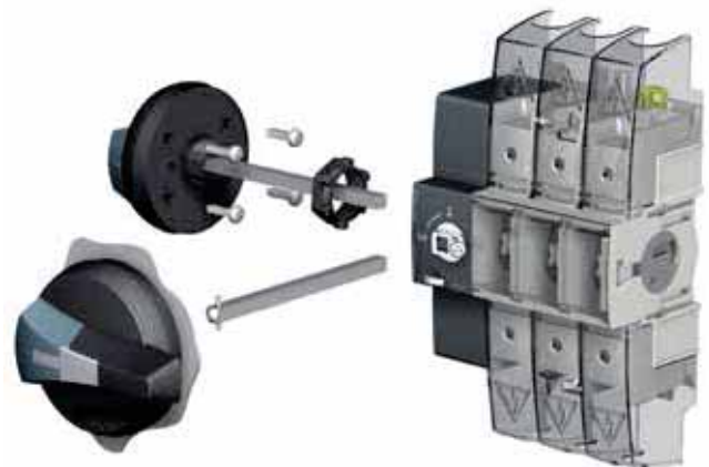
External front and left side operation
