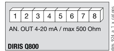
DIRIS Q800 1-2: analogue output 1 3-4: analogue output 2 5-6: analogue output 3 7-8: analogue output 4
