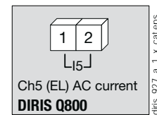
DIRIS Q800 1-2: differential core connections
