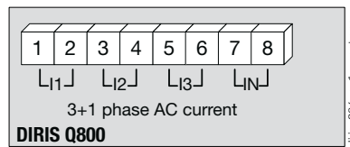
DIRIS Q800 1-2: current input i1 3-4: current input i2 5-6: current input i3 7-8: current input iN
